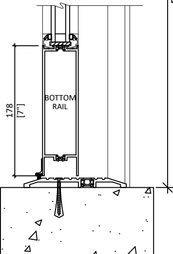
THERMAL PERFORMANCE DOOR CROSS SECTION
